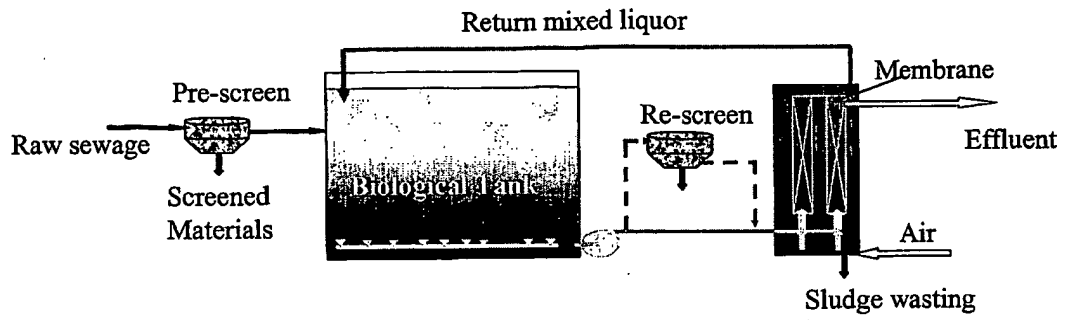
Figure 22 - MemJet MBR Configuration with Re-screening
